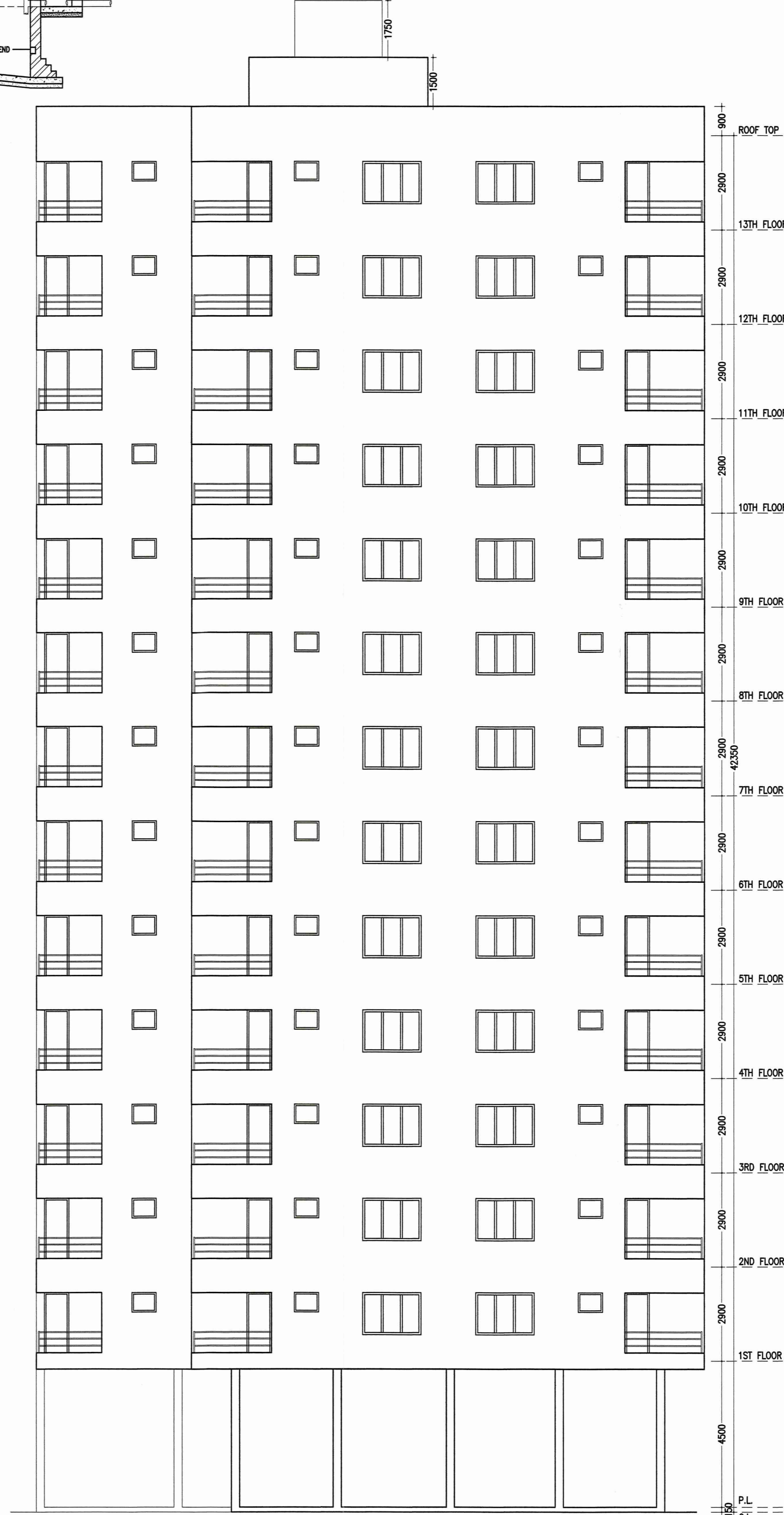
FRONT ELEVATION SCALE-1:100
