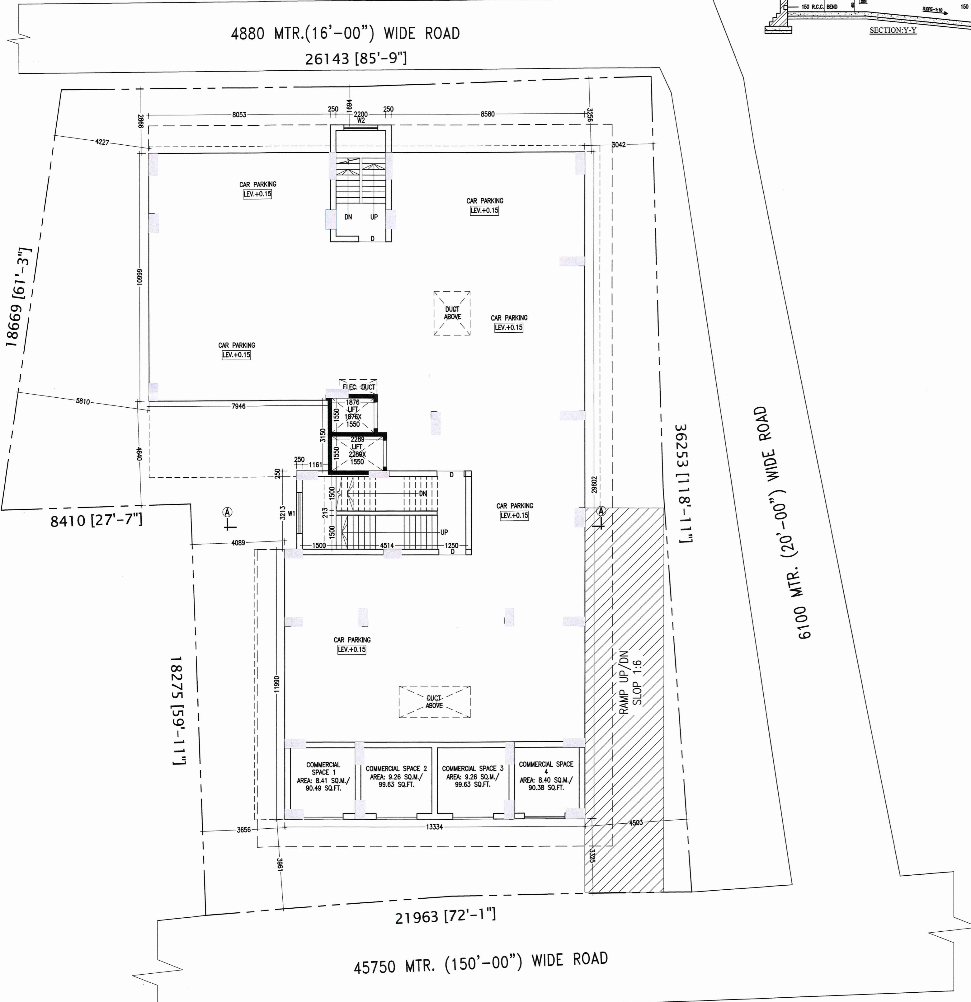
GROUND FLOOR PLAN SCALE-1:100
